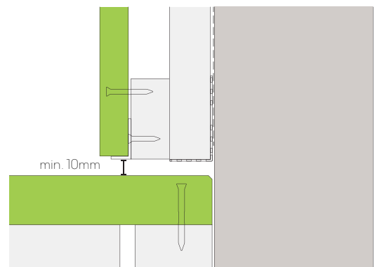
Fig. 5 - Install detail above deck
